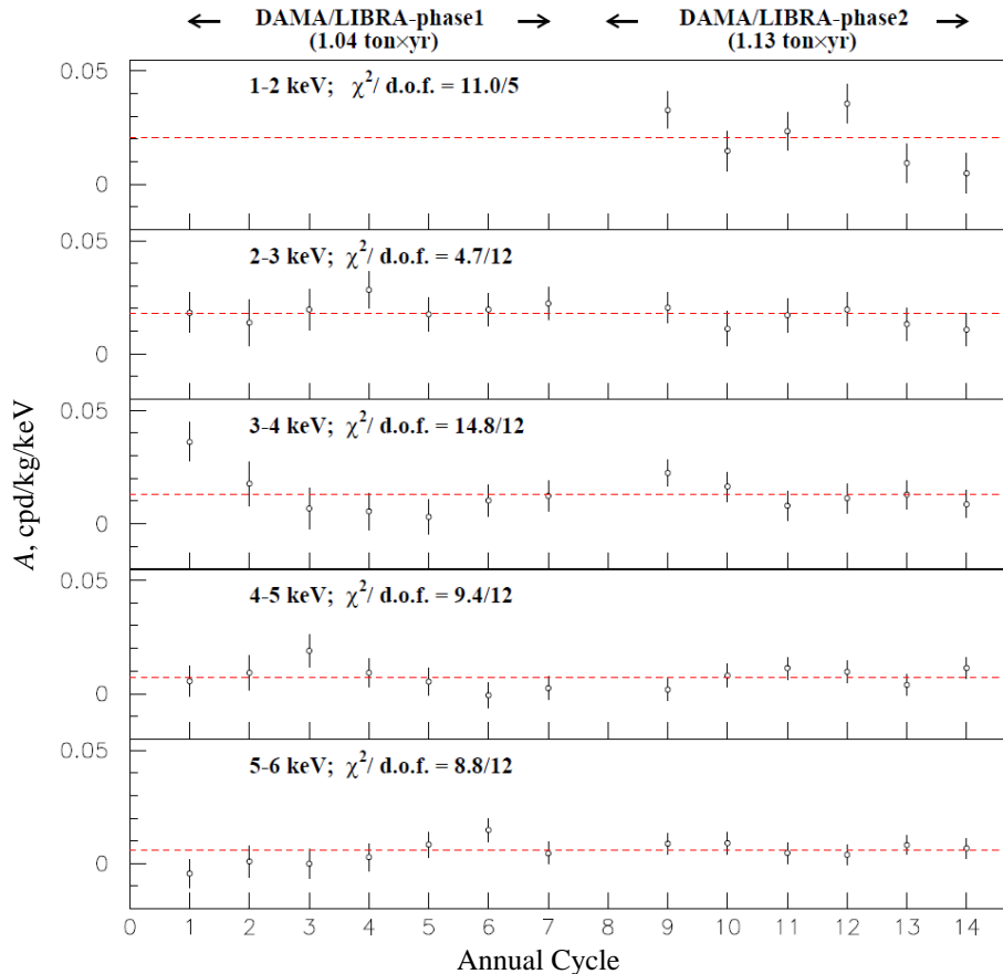
Fig. 14. Modulation amplitudes of each single annual cycle of DAMA/LIBRA-phase1 and DAMA/LIBRA-phase2. The error bars are the 1\sigma errors. The dashed horizontal lines show the central values obtained by best fit over the whole data set. The \chi^2 test and the run test accept the hypothesis at 95 % C.L. that the modulation amplitudes are normally fluctuating around the best fit values.
