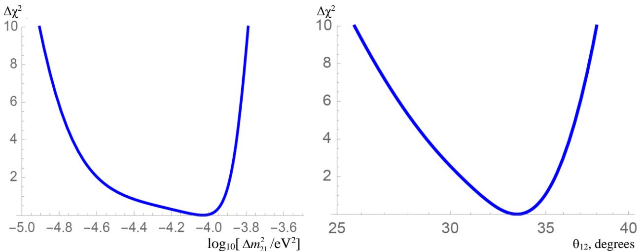
Fig. 3. One-dimensional \Delta\chi^2 distribution, for the analysis of the solar neutrino data based on the four known values of the survival probabilities summarized in the Table.
