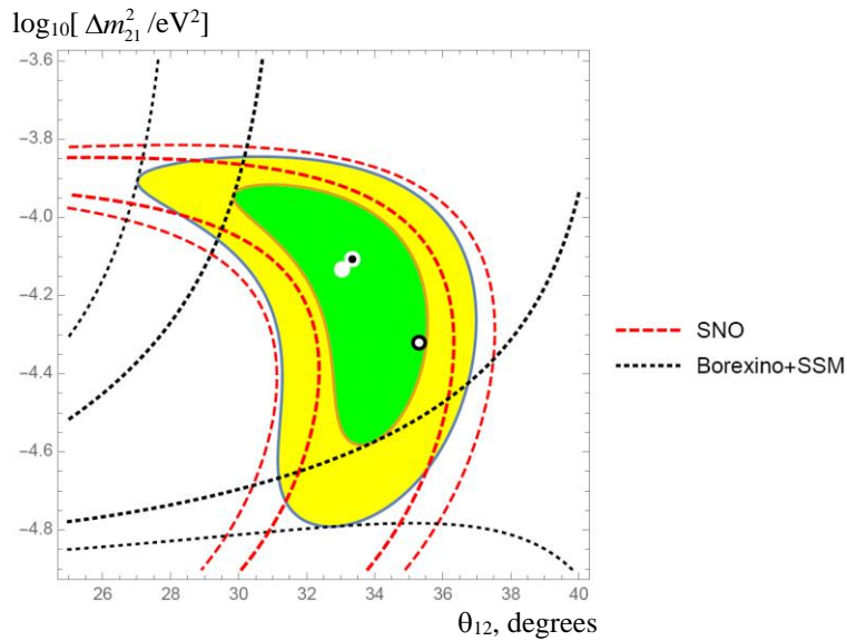
Fig. 2. The two-dimensional areas filled in green (yellow) enclose the 68.3 % (95 %) confidence regions of our solar neutrino analysis. We show separately the impact of the three values of the survival probability known at low energies (Borexino+SSM, dotted lines) and of the single value known at high energy (SNO, dashed lines). The three circles show three best fit points, given in Eq. (15): the best fit point of this analysis is given by the white disk dotted in black; the white disk indicates the best global fit value; the black disk dotted in white is the best global fit of Super-Kamiokande data alone. (See color Figure on the journal website.)
