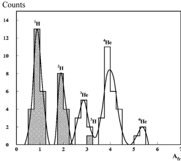
Fig. 4. Distribution by the mass number A_{fr} = p\beta c/p_0\beta_{0c} (where p\beta c is the experimentally obtained value, p_0 = 2.86A GeV/c, \beta_0 = 0.9 ) of single-charged (shaded histogram) and double-charged (non-shaded histogram) fragments for the fragmentation ^{14}N \rightarrow 3He + H and ^{14}N \rightarrow C + H channels.
