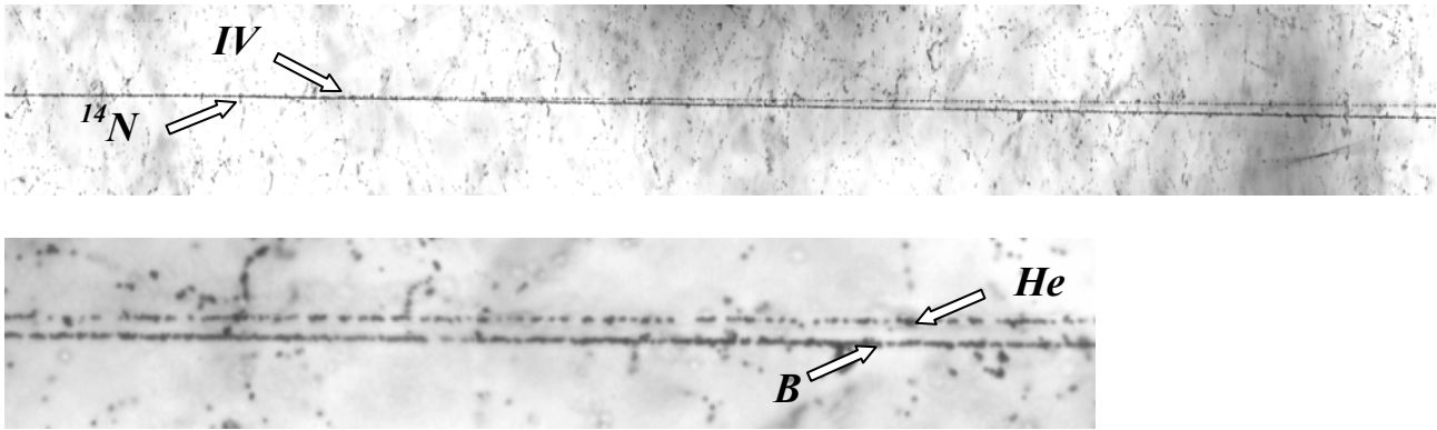
Fig. 2. Microphotograph of the nucleus fragmentation ^{14}\text{N} \rightarrow ^{10}\text{B} + ^4\text{He} at 2.1A GeV in peripheral interaction in emulsion. The upper photograph shows the interaction vertex IV and a narrow jet involving two fragments. In displacing along the fragment jet (lower photo) one sees clearly one multi-charged fragment with Z = 5 or ^{10}\text{B} and one double-charged fragment ^4\text{He} .
