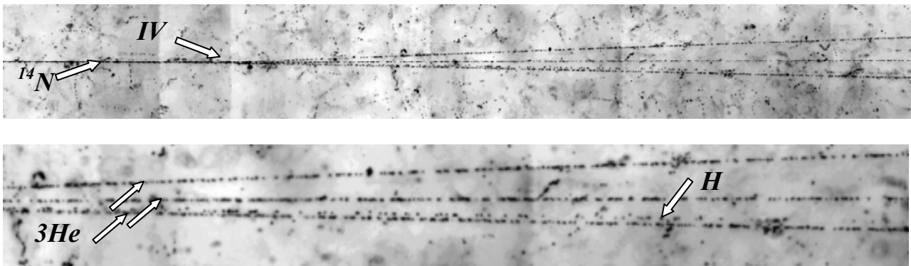
Fig. 1. Microphotograph of the nucleus fragmentation ^{14}\text{N} \rightarrow 3\text{He} + \text{H} at 2.1A GeV in peripheral interaction in emulsion. The upper photograph shows the interaction vertex without target fragment production and the fragment jet. In displacing along the fragment jet (lower photo) it is possible to see three double-charged ( He ) and one single-charged fragment ( H ).
