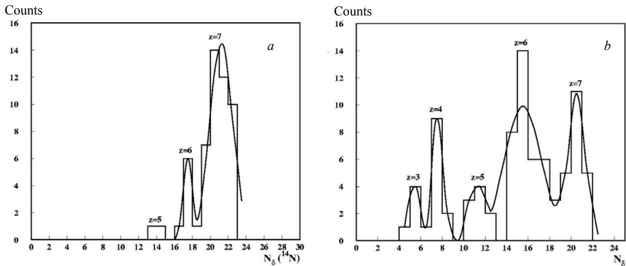
Fig. 3. Distribution by the \delta -electron number per 1 mm of the track on: a - primary ^{14}\text{N} nuclei; b - ^{14}\text{N} nucleus fragments with 3 - 7 charges. The continuous line is the description by the Gauss function sum.
