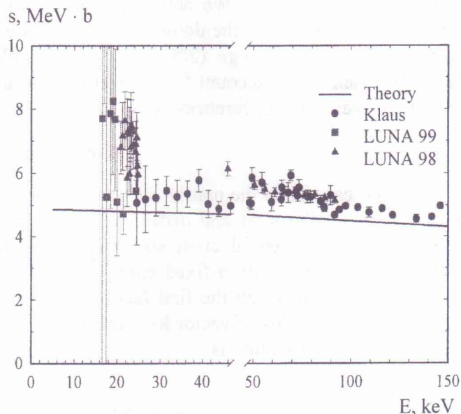
Fig. 3. S-factor of the reaction {}^3\text{He}({}^3\text{He}, 2p){}^4\text{He} . The experimental data are from [30] (Krauss), [9] (LUNA 99) and [7] (LUNA 98).
