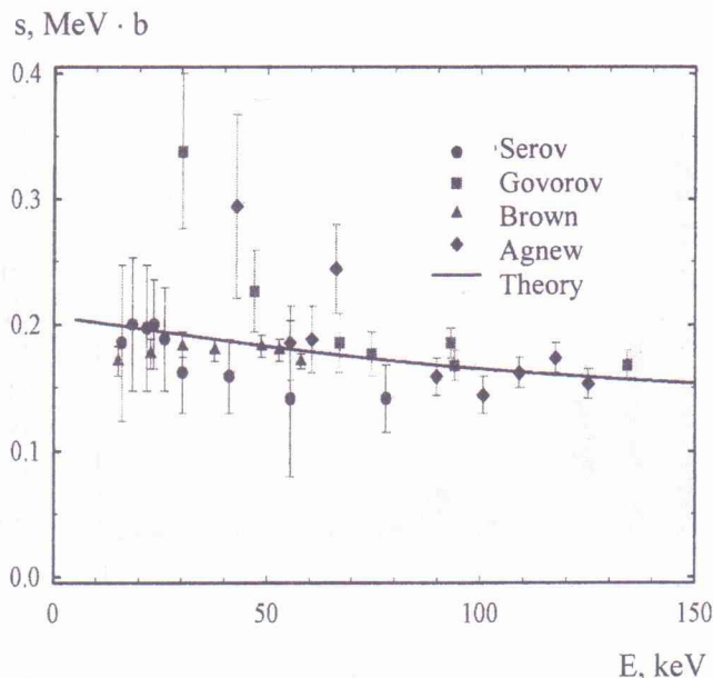
Fig. 2. S-factor of the reaction {}^3\text{H}({}^3\text{H}, 2n){}^4\text{He} . The experimental data are taken from [26] (Serov), [27] (Govorov), [28] (Brown) and [29] (Agnew).
