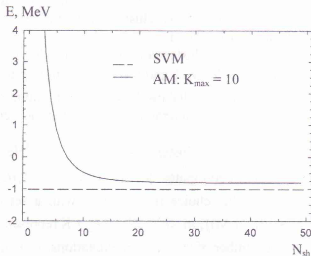
Fig. 1. Ground state of {}^6\text{He} as a function of the number of oscillator shells in the AM tree-cluster model compared to the results of [19]. The energy is relative to the protect \alpha + n + n threshold.
