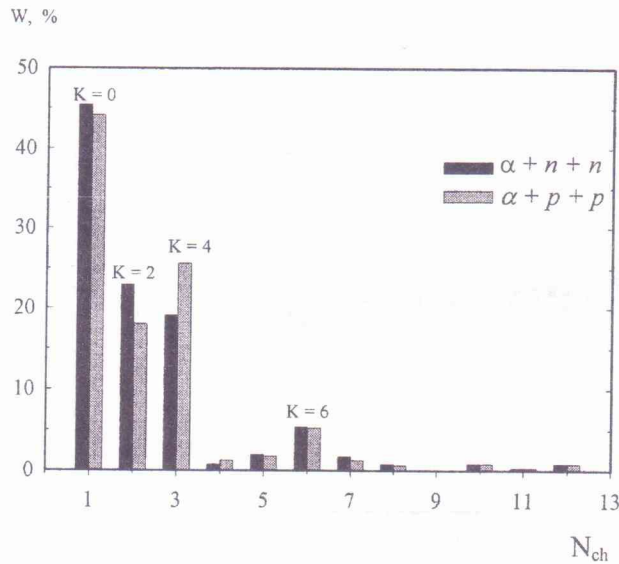
Fig. 4. Contribution of three-cluster channels to the total s-factor of the reactions {}^3\text{H}({}^3\text{H}, 2n){}^4\text{He} and {}^3\text{He}({}^3\text{He}, 2p){}^4\text{He} in a full calculation with K_{\text{max}} = 10 .
