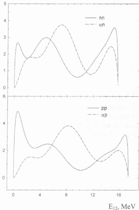
Fig. 5. Partial differential cross sections of the reactions {}^3\text{H}({}^3\text{H}, 2n){}^4\text{He} and {}^3\text{He}({}^3\text{He}, 2p){}^4\text{He} .
