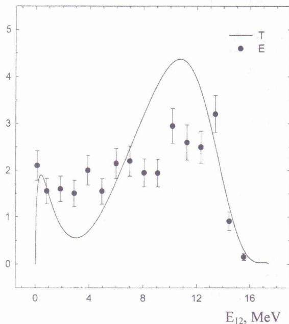
Fig. 6. Calculated and experimental differential cross section for the reaction {}^3\text{He}({}^3\text{He}, 2p){}^4\text{He} . Experimental data is taken from [25].
